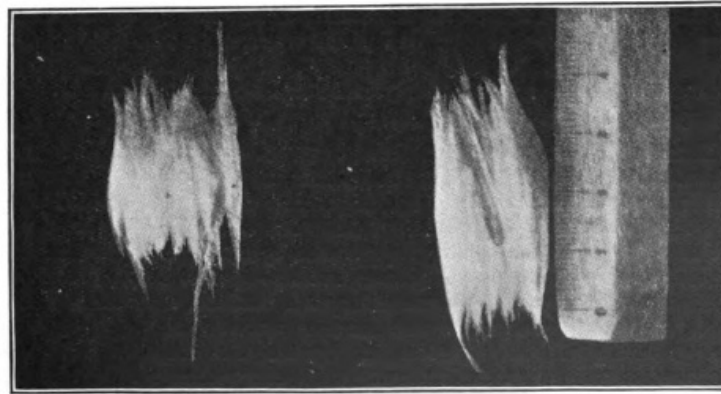
Figure A.9: A comparison of ginned (left) and hand-cleaned cotton (right) fiber length
