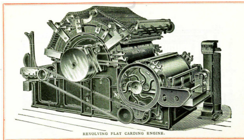
Figure A.7: Dobson & Barlow Carding Machine circa 1920
