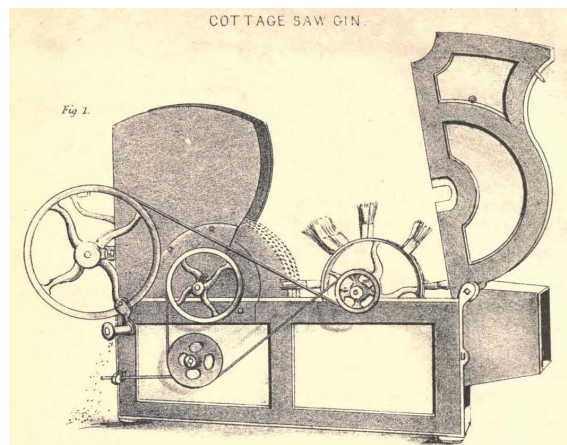
Figure A.4: Cottage Saw Gin
