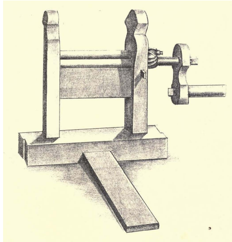
Figure A.3: Indian Churka for removing cotton seeds
